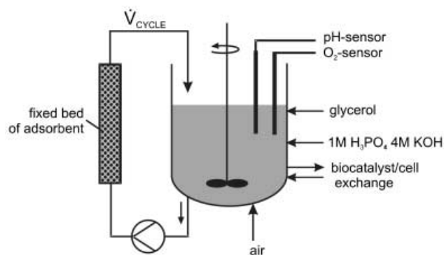
Scheme 3. Recycle reactor with fixed bed of adsorbent in external loop.
