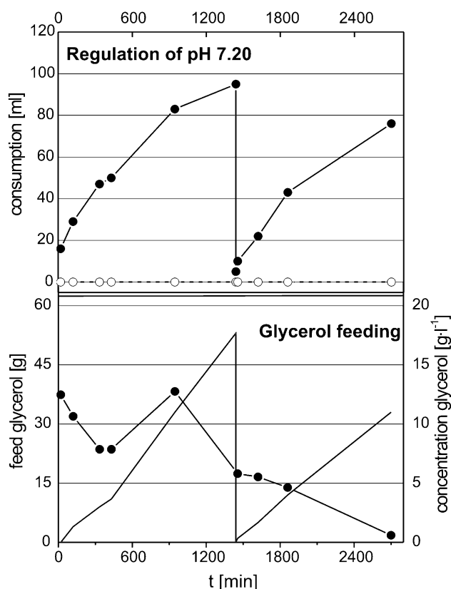
Figure 8. Baeyer–Villiger oxidation of rac - 1 in the 1-L bubble column. Upper diagram: Regulation at pH 7.2 with —●— 1 M H 3 PO 4 [mL] and —●— 4 M KOH [mL]. Lower diagram: Glycerol availability. —●— glycerol concentration in cell broth [g L -1 ], —○— glycerol feed [g].
