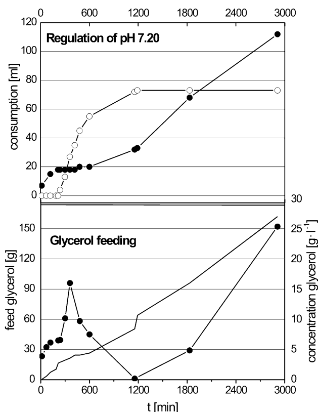
Figure 7. Baeyer–Villiger oxidation of rac - 1 in the recycle reactor. Upper diagram: Regulation at pH 7.2 with —●— 1 M H 3 PO 4 [mL] and —●— 4 M KOH [mL]. Lower diagram: Glycerol availability. —●— glycerol concentration in cell broth [g L -1 ], —○— glycerol feed [g].
