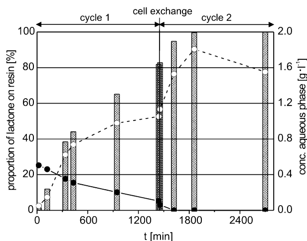
Figure 6. Baeyer–Villiger oxidation of 25 g of rac - 1 in the 1-L bubble column over two cycles: Exchange of biocatalyst after 24 hours. ▨ proportion of re-adsorbed combined lactones ( 2 and 3 ) extracted from a resin sample, (●) ketone concentration and (○) lactone concentration of the cell broth.
