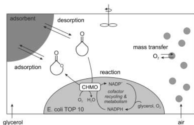
Scheme 2. Principle of the “two-in-one” resin-based in situ SFPR process for microbial Baeyer–Villiger oxidation.
