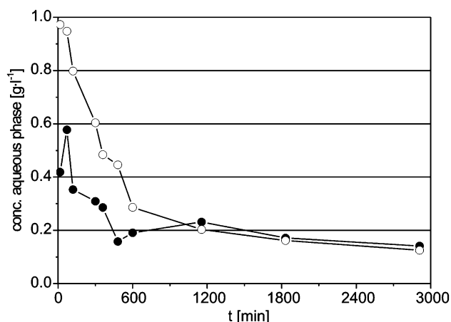
Figure 4. Baeyer–Villiger oxidation of rac - 1 in a recycle reactor: (○) ketone concentration in feed and (●) in the fermenter.
