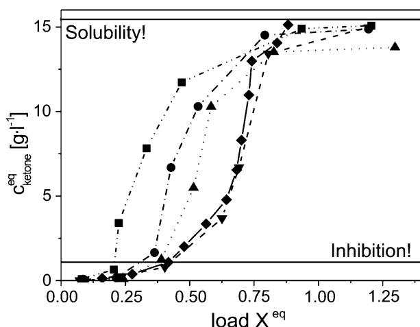
Figure 2. Adsorption equilibria of bicyclo[3.2.0]hept-2-ene-6-one ( 1 ) on different materials (S-shaped curves). Liquid phase concentration c_{\text{ketone}}^{\text{eq}} in dependence of the equilibrium load X^{\text{eq}} . (■) active charcoal Norit Darco, (●) active charcoal, (▲) active charcoal Norit RO 0.8, (▼) Lewatit VPOC1163, (◆) Optipore L-493.
