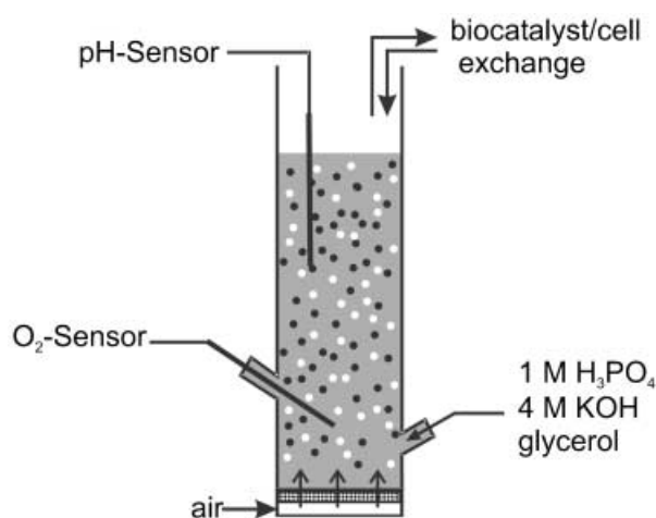
Scheme 4. Scheme of a “bubble column” set-up.
