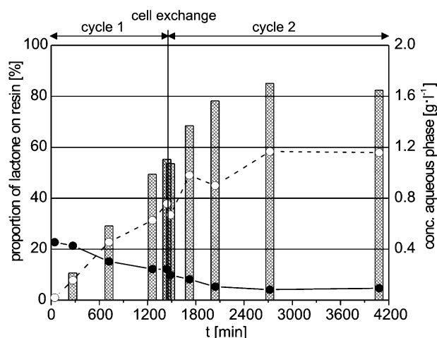
Figure 3. Baeyer–Villiger oxidation of 25 g of rac - 1 in a 1-L fermenter over two cycles (exchange of biocatalyst after 24 hours). ▨ proportion of readsorbed combined lactones extracted from a resin sample, ● ketone and ○ lactone concentration in the cell broth.
