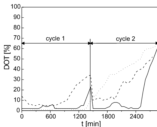
Figure 9. Dissolved oxygen profiles in the different reactor in — fermenter, ···· recycle reactor, — — — bubble column.
