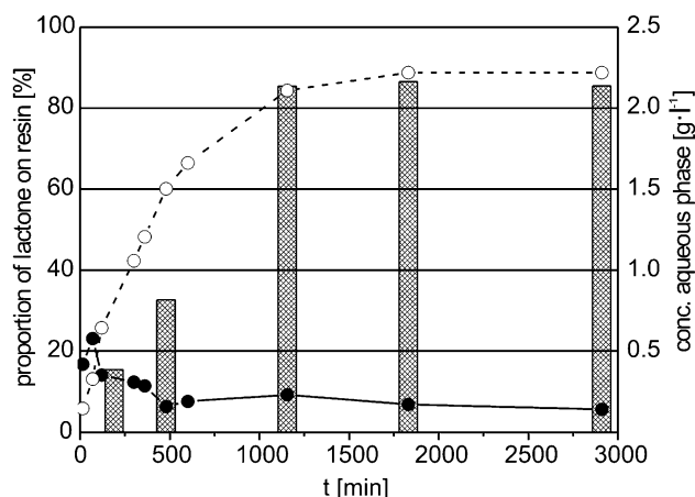
Figure 5. Baeyer–Villiger oxidation of 25 g of 1 in a 1-L recycle reactor (without change of biocatalyst). ▨ proportion of readsorbed combined lactones extracted from a resin sample, (●) ketone concentration and (○) lactone concentration of the cell broth inside the fermenter.
