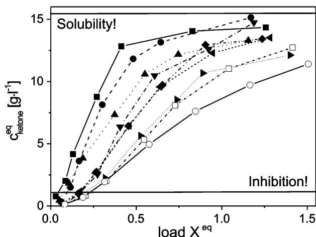
Figure 1. Adsorption equilibria of bicyclo[3.2.0]hept-2-ene-6-one ( 1 ) on different materials ( \Gamma -shaped curves): Liquid phase concentration c_{\text{ketone}}^{\text{eq}} in dependence of the equilibrium load X^{\text{eq}} . (■) Duolite S761, (●) Amberlite XAD2, (▲) Amberlite XAD7, (▼) Sepabeads SP207, (◆) Amberlite XAD1180, (◄) Optipore L-323, (◄) Amberlite XAD4, (□) Lewatit VPOC1064, (○) Amberlite XAD16.
