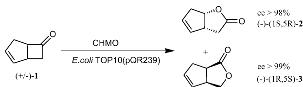
Scheme 1. Microbial Baeyer–Villiger oxidation of rac -bicyclo[3.2.0]hept-2-en-6-one ( 1 ).
